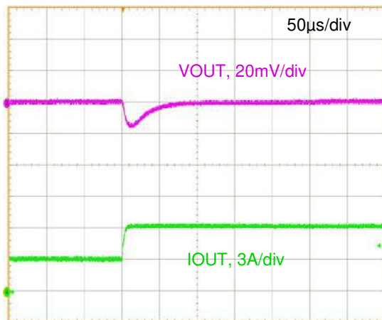
Figure 27. Step Load Transient Response (VIN=12V, VOUT=0.7V, COUT=200μF, IOUT=3 to 6A, 1.0A/μs)
