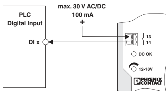
Figure 18 Wiring principle
