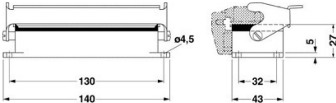
Dimensioned drawing
