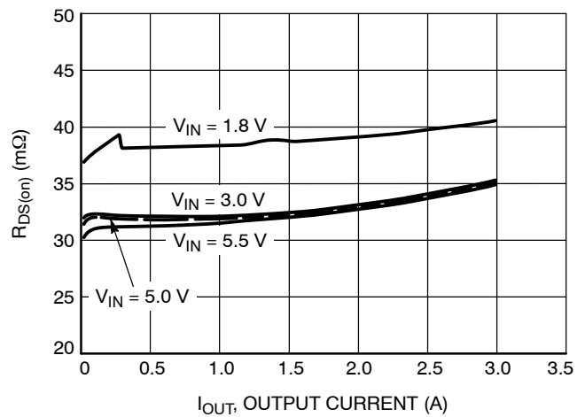
Figure 8. R_{DS(on)} vs. I_{OUT} at 25^\circ\text{C}
