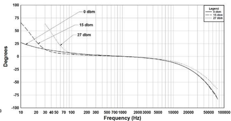
108J Rs=1000, RI=600 Phase Shift
