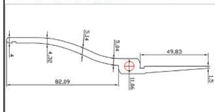
BENT NOSE 6" WITH SMOOTH JAWS
