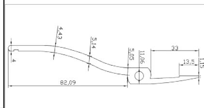
LONG NEEDLE NOSE 6" WITH SERRATED JAWS
