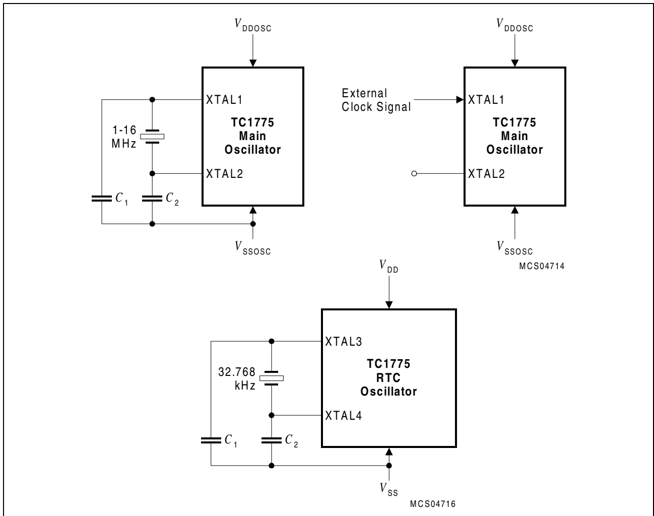
Figure 19 Oscillator Circuitries
