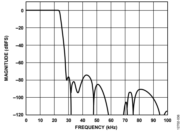
Figure 36. Total Decimation Response, f_s = 192 kHz, Serial Port f_s = 48 kHz
