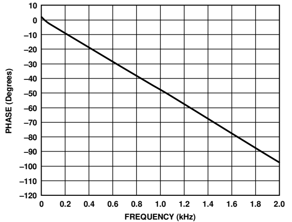
Figure 24. Phase vs. Frequency, 2 kHz Bandwidth, f_s = 48 kHz, Signal Path = DAC_SDATA to ASRC to LOU TLx
