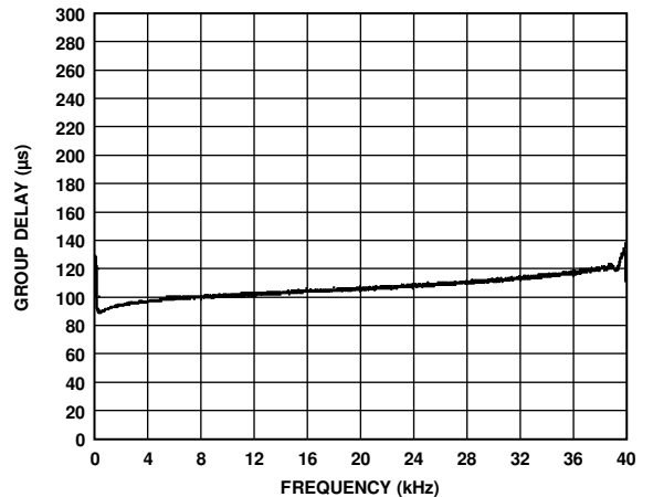
Figure 25. Group Delay vs. Frequency, f_s = 96 kHz, Signal Path = DAC_SDATA to ASRC to LOU TLx
