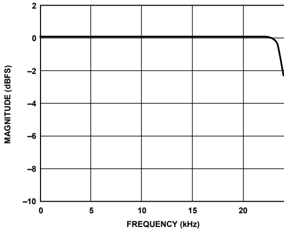
Figure 33. Decimation Pass Band Response, f_s = 96 kHz
