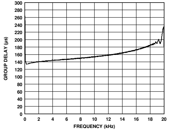
Figure 23. Group Delay vs. Frequency, f_s = 48 kHz, Signal Path = DAC_SDATA to ASRC to LOU TLx
