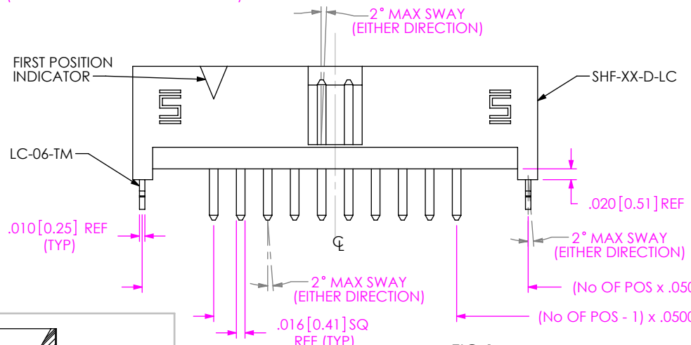
FIG 1 (SHF-110-01-X-D-TH-LC SHOWN)
