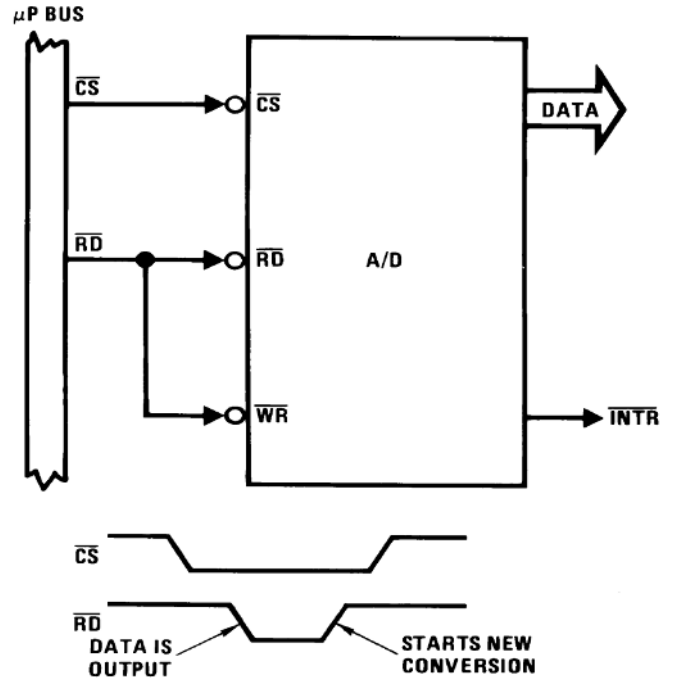
Figure 69. Read-Only Interface
