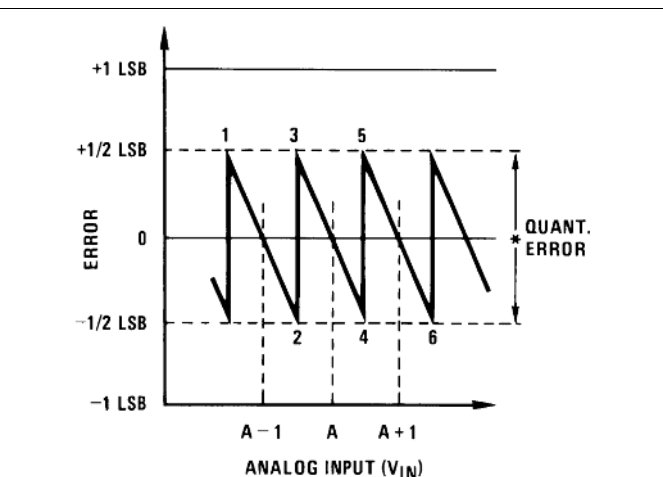
Figure 17. Clarifying the Error Specs of an ADC Converter Accuracy=±0 LSB: A Perfect ADC
