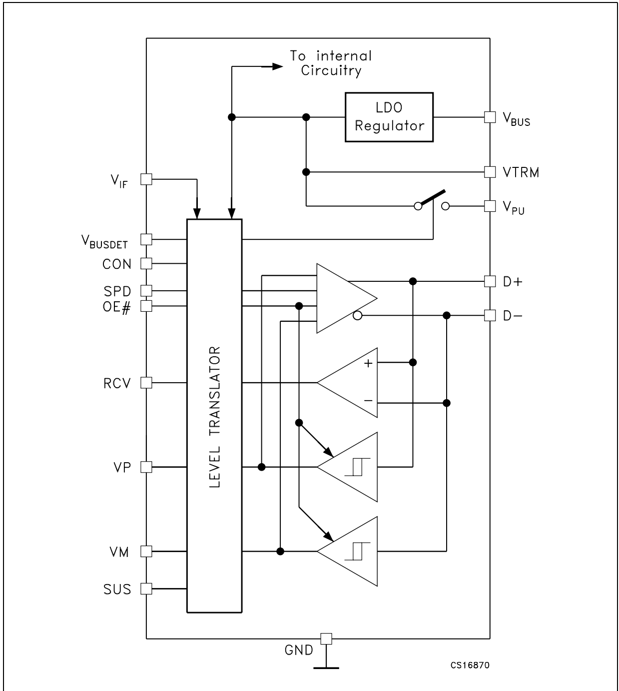
Figure 10. Functional diagram
