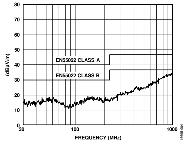
Figure 4. Vertical Scan from 30 MHz to 1 GHz with 50 mA, 5 V Output
