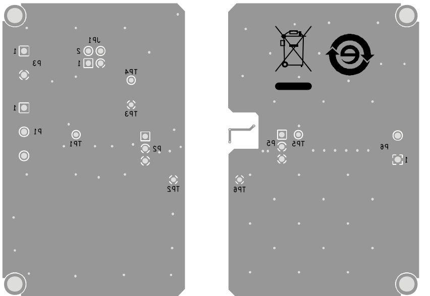
Figure 7. EVAL-ADuM5028EBZ Evaluation Board Bottom Layer and Silkscreen
