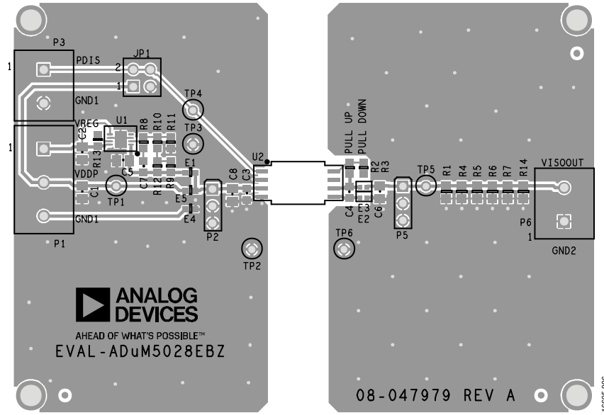
Figure 6. EVAL-ADuM5028EBZ Evaluation Board Top Layer and Silkscreen
