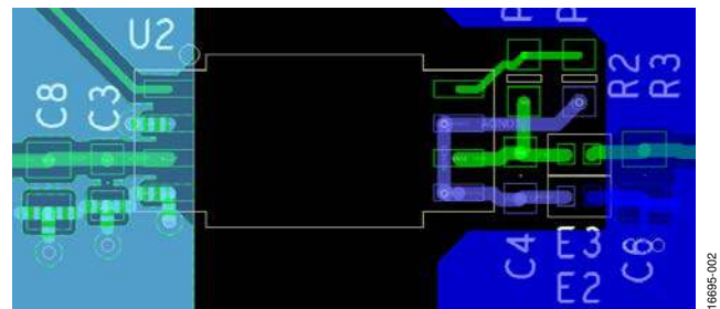
Figure 2. Layout Guidelines for EVAL-ADuM5028EBZ
