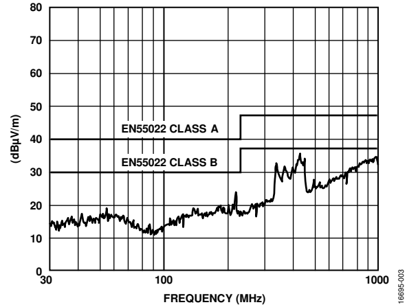
Figure 3. Horizontal Scan from 30 MHz to 1 GHz with 50 mA, 5 V Output
