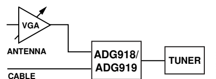
Figure 28. Tuner Modules
