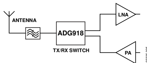
Figure 27. Wireless Metering
