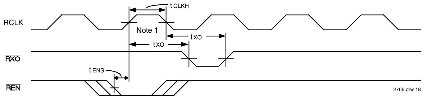
Figure 16. Read Expansion Out Timing
