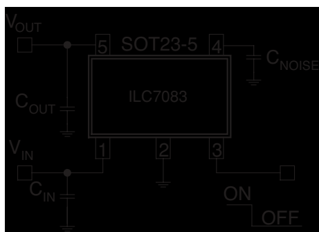
Figure 4. Basic Application Circuit for Fixed Output Voltage Versions
