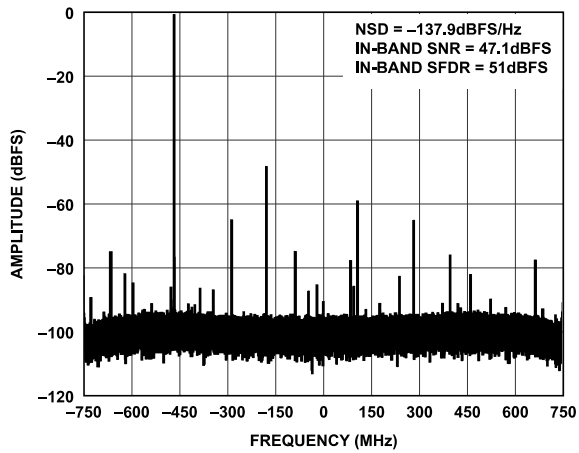
Figure 49. Single-Tone FFT at f_{IN} = 6300 MHz
