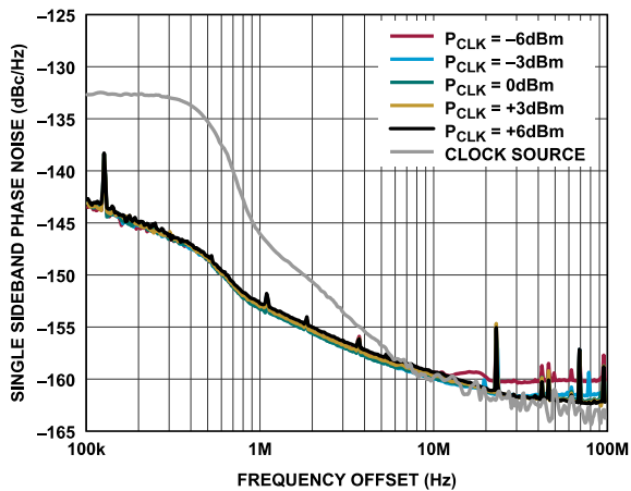
Figure 25. Single Sideband Phase Noise vs. Frequency Offset for Different Clock Input Power ( P_{CLK} ), f_{OUT} = 1.8 \text{ GHz} , External 12 GHz Clock Input with Clock PLL Disabled
