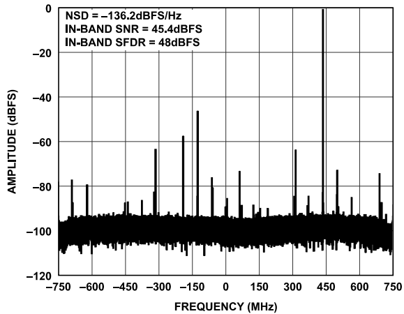
Figure 50. Single-Tone FFT at f_{IN} = 7200 MHz
