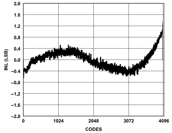
Figure 75. INL, f_{IN} = 255 MHz
