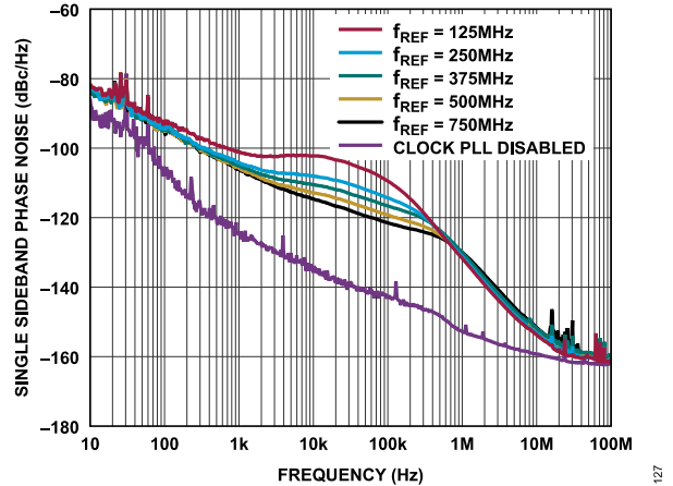
Figure 27. Single Sideband Phase Noise vs. Frequency Offset for Different PLL Reference Clocks ( f_{REF} ), f_{OUT} = 1.8 \text{ GHz} , f_{DAC} = 12 \text{ GSPS} , PLL Enabled with Exception of External 12 GHz Clock Input with Clock PLL Disabled
