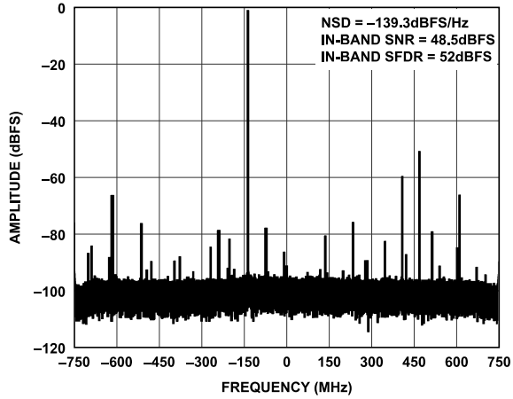
Figure 48. Single-Tone FFT at f_{IN} = 5400 MHz
