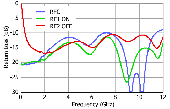
Return Loss
