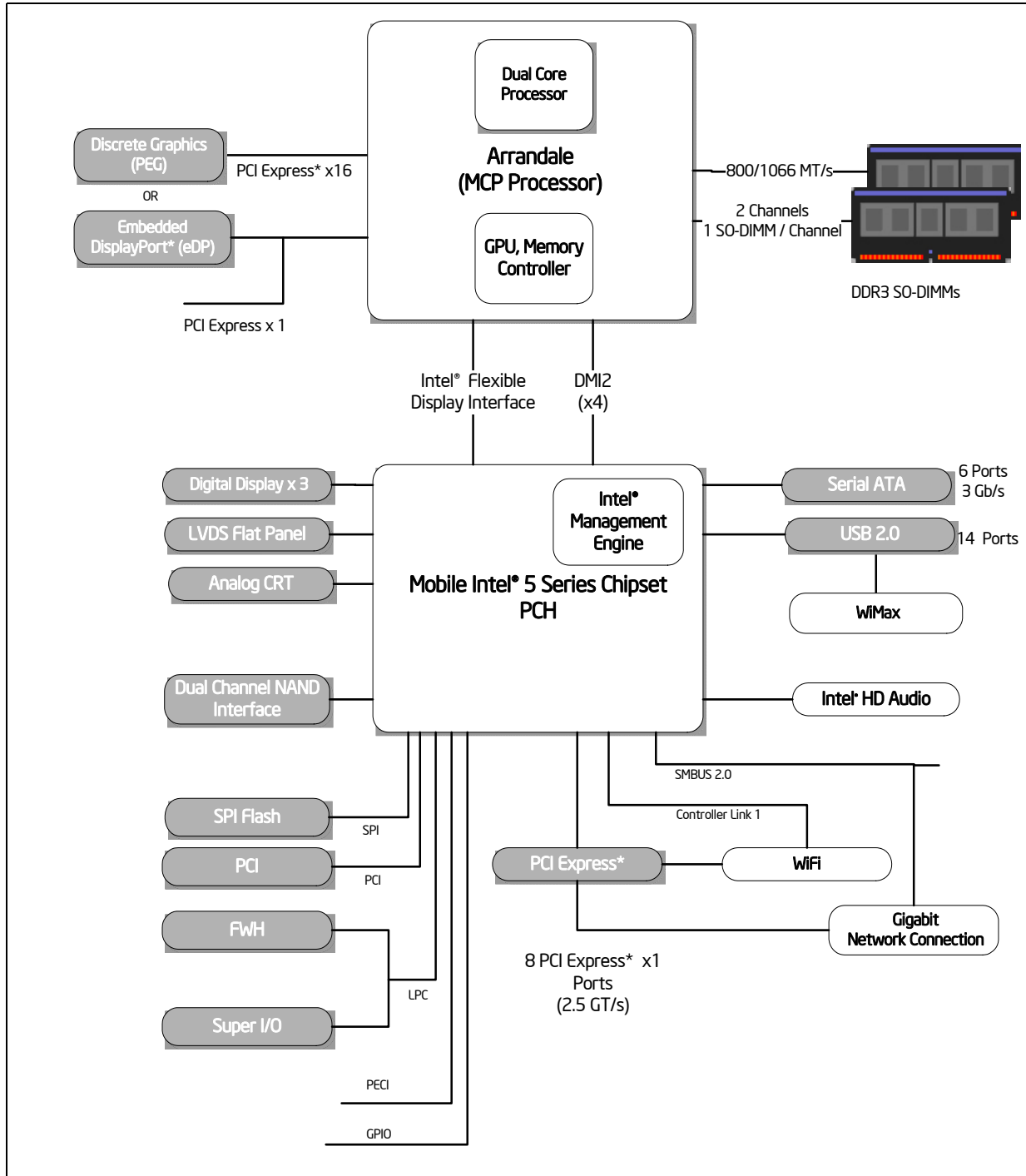
Figure 1. Intel® Celeron™ P4000 and U3000 mobile processor series on the Galpella Platform
