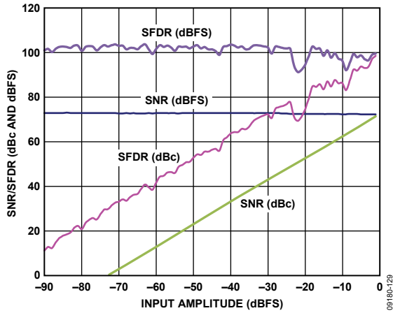
Figure 29. AD9644-155 Single-Tone SNR/SFDR vs. Input Amplitude ( A_{IN} ) with f_{IN} = 10.1 MHz, f_S = 80 MSPS
