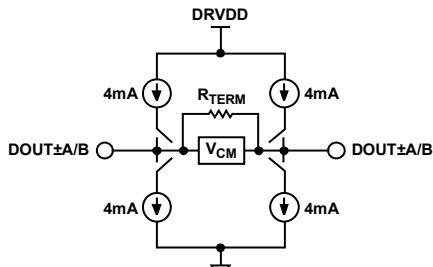
Figure 43. Digital CML Output
