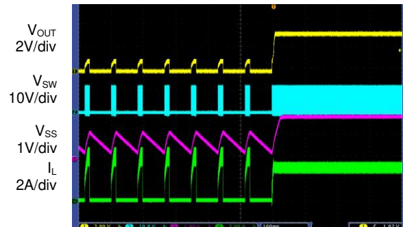
Time 100ms/div
