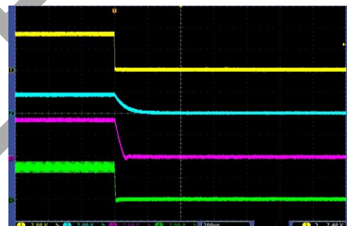
Time 200µs/div
