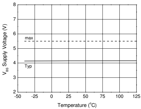
Figure 25a. VBS UnderVoltage Threshold (+) vs Temperature
