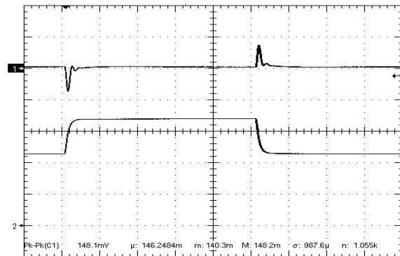
Figure 12. Load Transient Response (100mV/div), di/dt=0.1A/uS, 50%-75%-50% of full load, Cout=Fig16 time scale: 200uS/div. Ch1=Vout, Ch2=Iout (2A/div)
