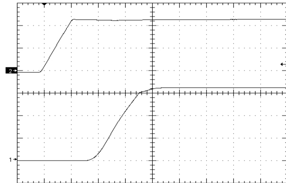
Figure 10. Startup Waveform via Input Voltage, time scale 2mS/div. Vin=Vin_nom, Iout=full load Cout=4700uF, Ch1=Vout (1V/div), Ch2=Vin (10V/div)
