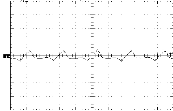
Figure 8. Output Voltage Ripple (20mV/div), time scale – 1uS/div. Vin=Vin_nom, full load Cout=1uF ceramic + 10uF Tantalum (see Fig 16)
