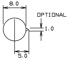
PANEL MOUNTING HOLE
