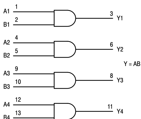
Figure 1. Logic Diagram
