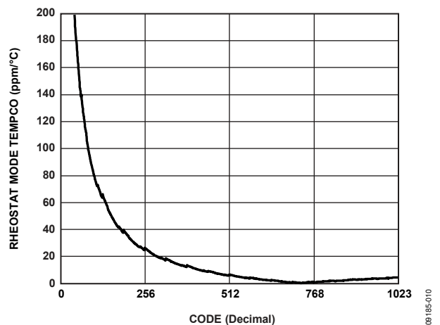
Figure 10. (\Delta R_{WB}/R_{WB})/\Delta T \times 10^6 Rheostat Mode Tempco
