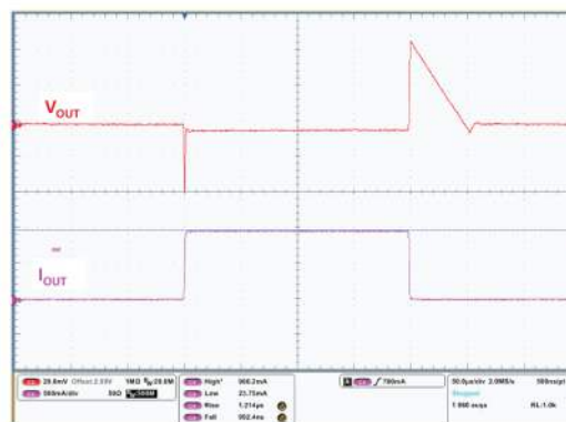
Figure 24. Load transient ( V_{IN} = V_{EN} = 3.5\text{ V} ; t_{RISE} = 1\text{ }\mu\text{s} ; I_{OUT} = 1\text{ mA} to 1\text{ A} )
