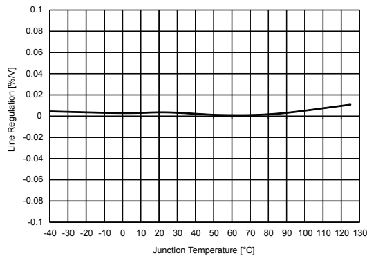
Figure 6. Line regulation vs. temperature ( V_{OUT} = 3.0 V , I_{OUT} = 1 \text{ mA} )
