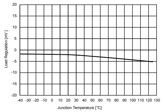
Figure 7. Load regulation vs. temperature ( V_{OUT} = 3.0 V , I_{OUT} = 1 \text{ A to } 10 \text{ mA} )
