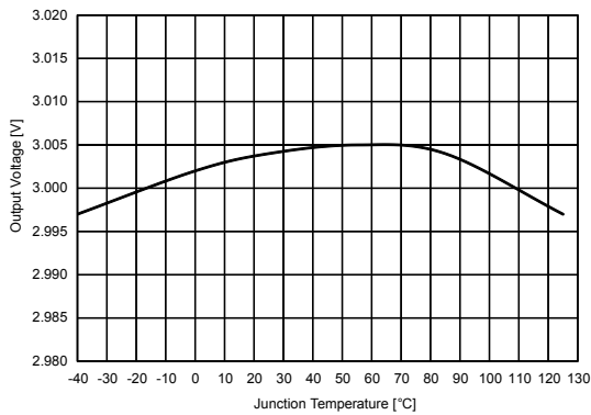
Figure 4. Output voltage vs. temperature ( V_{IN} = 3.0 V , I_{OUT} = 1 \text{ mA} , normal mode)
