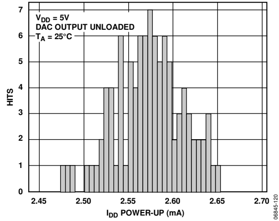
Figure 19. I_{DD} Histogram V_{DD} = 5.5 V
