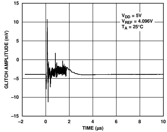
Figure 31. Digital Crosstalk
