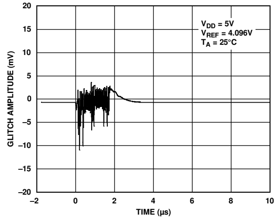
Figure 32. DAC-to-DAC Crosstalk
