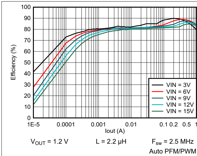
Figure 9-38. Efficiency vs Output Current
