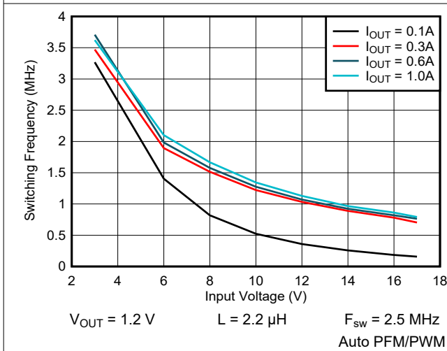
Figure 9-40. Switching Frequency vs Input Voltage
