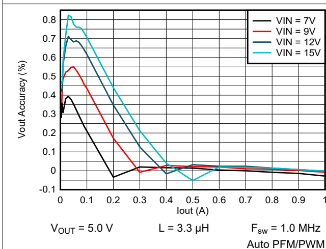
Figure 9-12. Output Voltage vs Output Current
