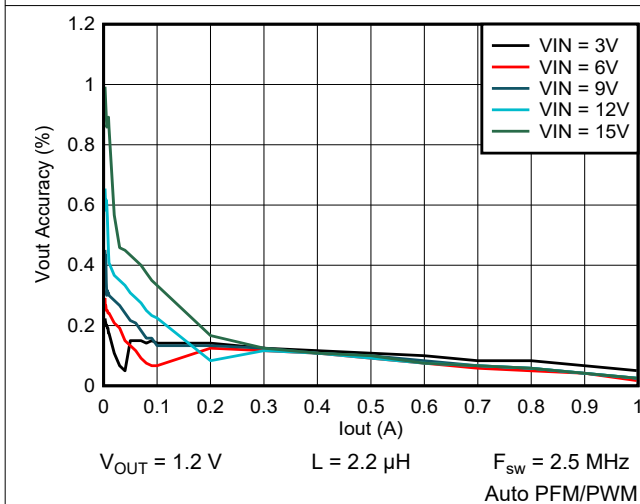
Figure 9-42. Output Voltage vs Output Current
