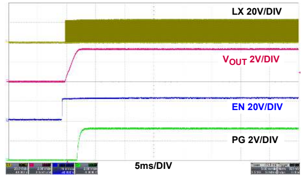
FIGURE 20. START-UP AT NO LOAD, PWM
