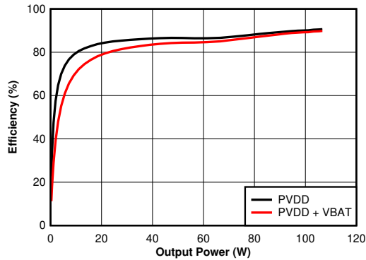
2 \Omega T_C = 75^\circ\text{C} PBTL Figure 6-22. Efficiency vs Output Power - PBTL, 2 \Omega
