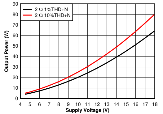
2 \Omega T_C = 75^\circ\text{C} PBTL Figure 6-21. Output Power vs Supply Voltage - PBTL, 2 \Omega
