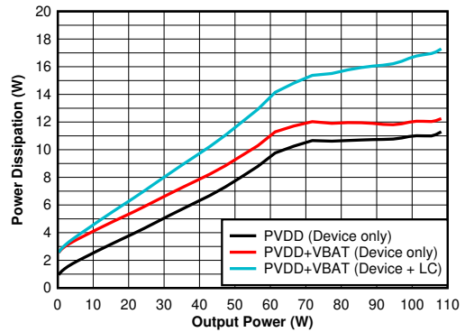
2 \Omega T_C = 75^\circ\text{C} PBTL Figure 6-23. Power Dissipation vs Output Power - PBTL, 2 \Omega
