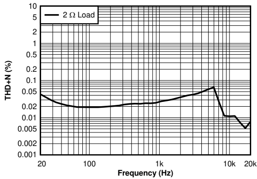
P_O = 1\text{ W} PBTL Figure 6-20. THD+N vs Frequency - PBTL, 2 \Omega
