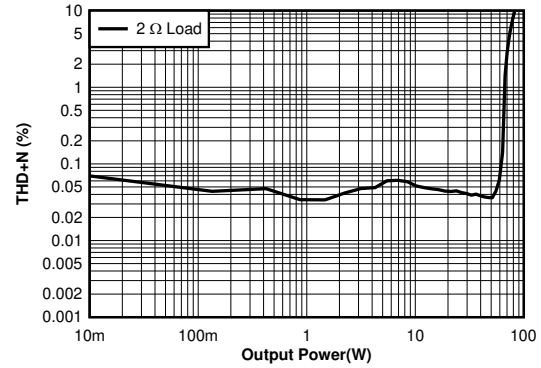
PVDD = 18 V PBTL Figure 6-19. THD+N vs Power - PBTL, 2 \Omega , 18 V
