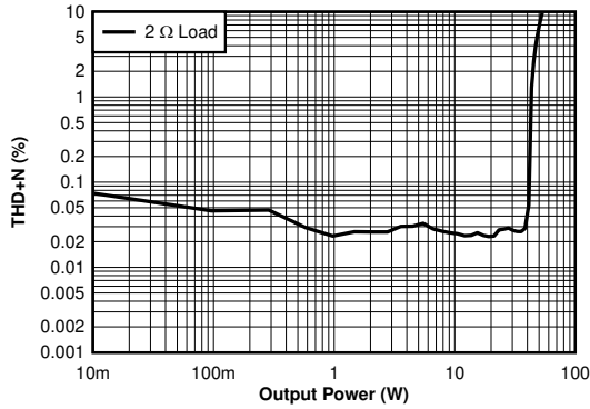
PVDD = 14.4 V PBTL Figure 6-18. THD+N vs Power - PBTL, 2 \Omega , 14.4 V
