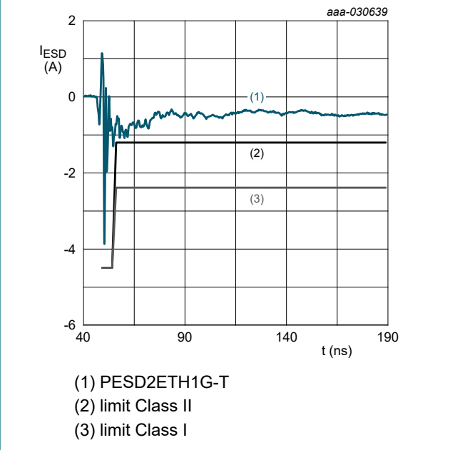
Fig. 29. ESD discharge current at -15 kV
