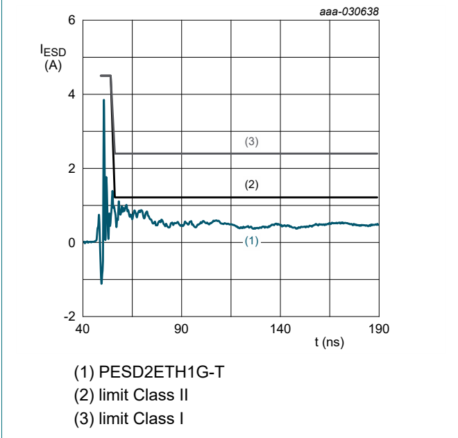
Fig. 28. ESD discharge current at +15 kV
