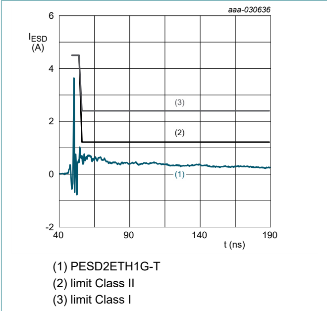
Fig. 26. ESD discharge current at +8 kV
