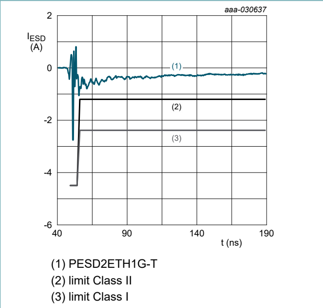
Fig. 27. ESD discharge current at -8 kV
