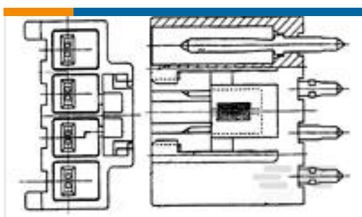
TE Part #1-178489-1 UP 3.96 6P TAB HDR NAT TYPE 2
