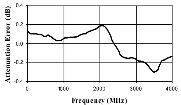
Attenuation Error, 1 dB Bit
