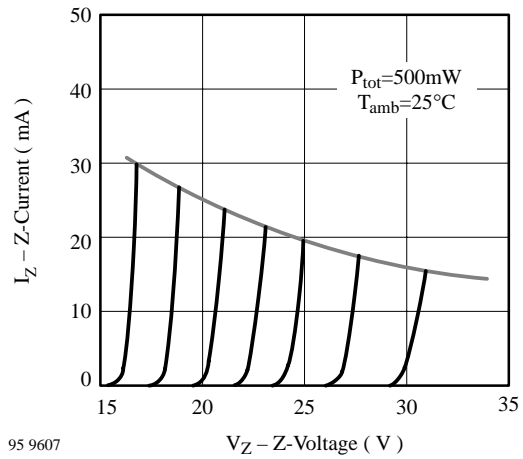
95 9607 Figure 9. Z-Current vs. Z-Voltage
