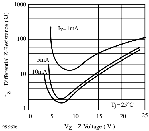
95 9606 Figure 10. Differential Z-Resistance vs. Z-Voltage
