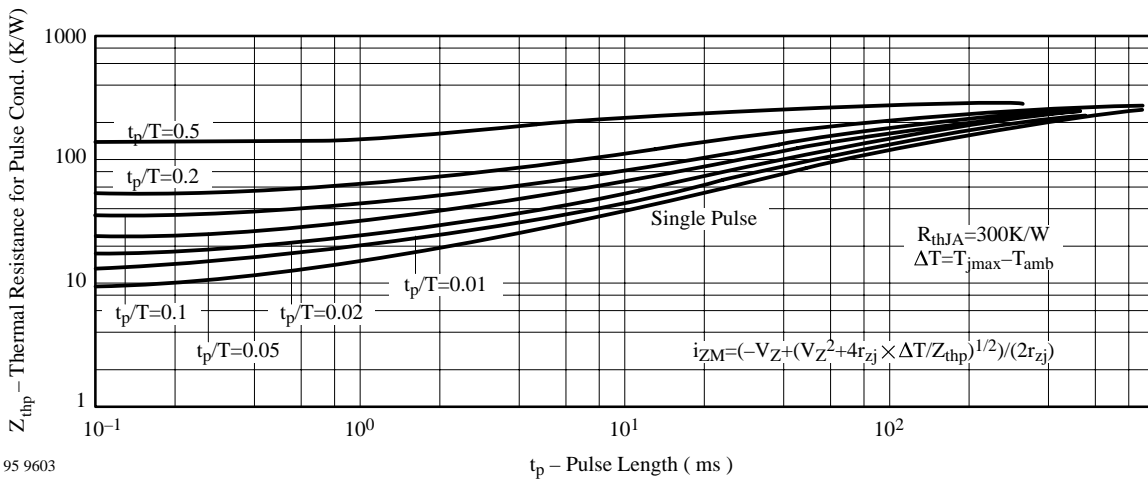
95 9603 Figure 11. Thermal Response
