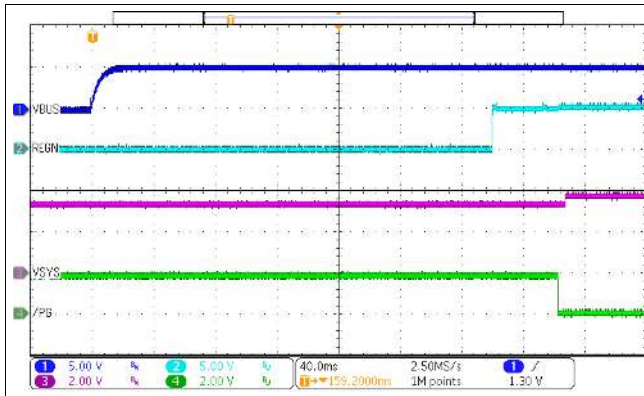
Figure 50. Power Up with Charge Disabled
