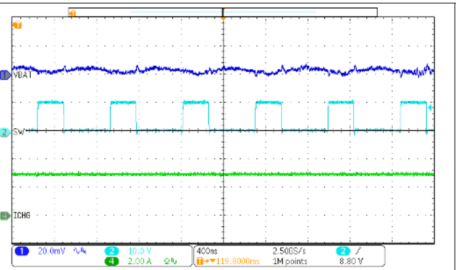
Figure 63. PWM Switching Waveform
