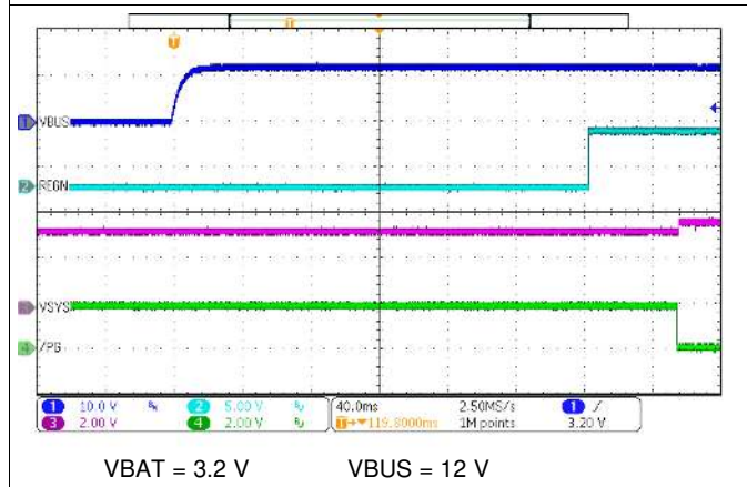
Figure 60. Power Up with Charge Disabled
