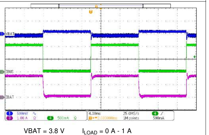
Figure 59. Boost Mode Load Transient
