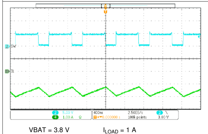
Figure 58. Boost Mode Switching Waveform
