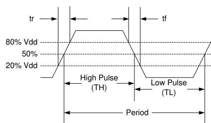
Figure 3. Waveform [10]
