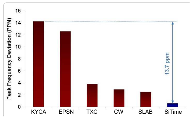
Figure 6. Shock Robustness [6]
