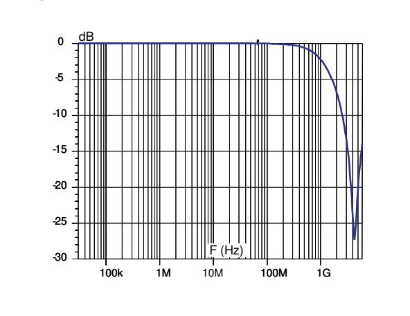
Figure 13: S21 attenuation measurement result
