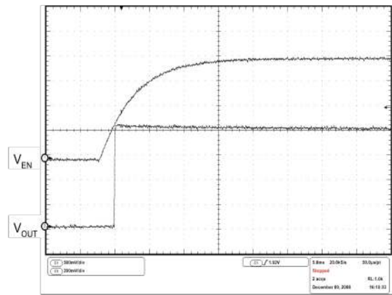
Figure 17. Enable transient
