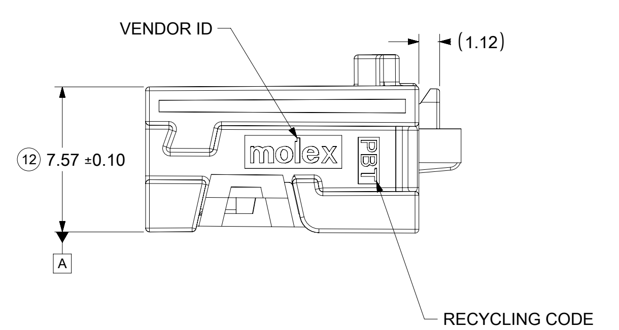
8CKT HINGE CLOSED CPA IN FINAL POSITION
