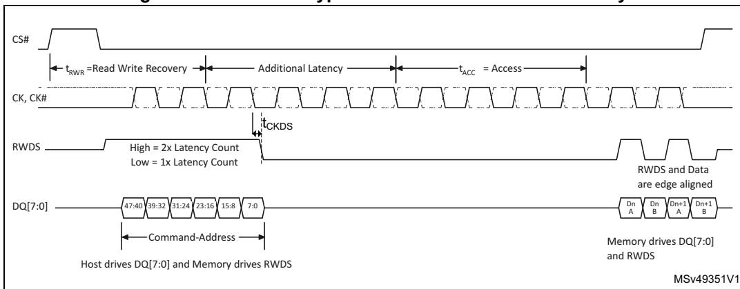
Figure 64. OCTOSPI HyperBus™ read with double latency
