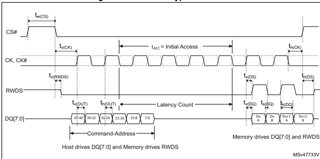
Figure 63. OCTOSPI HyperBus™ read
