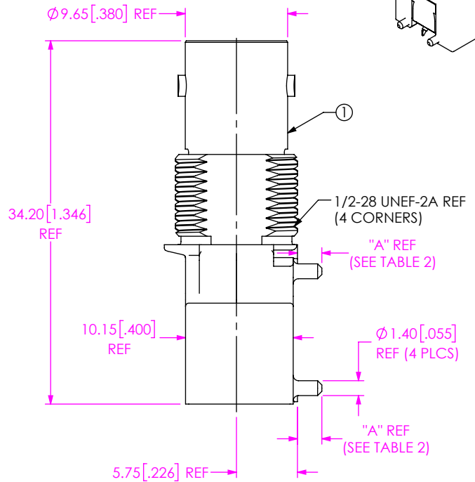
FIG 1 BNC7T-J-P-XX-RA-BM1D SHOWN
