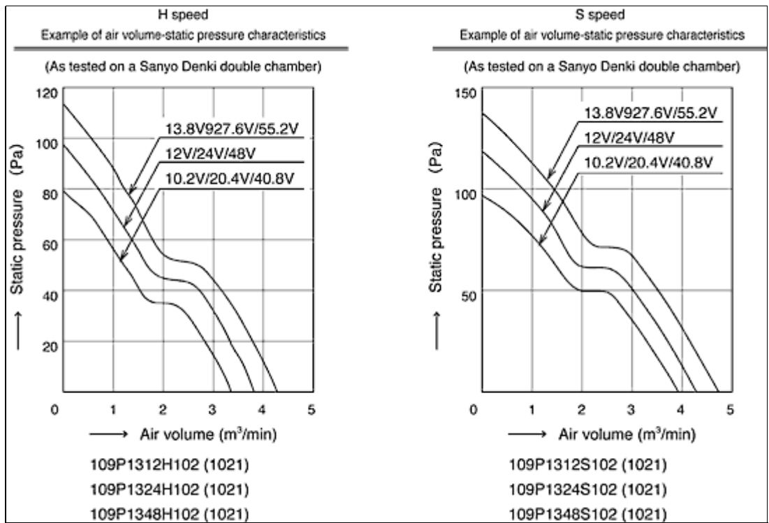
fig.3 Air volume-static pressure characteristics of "SAN ACE 127"
