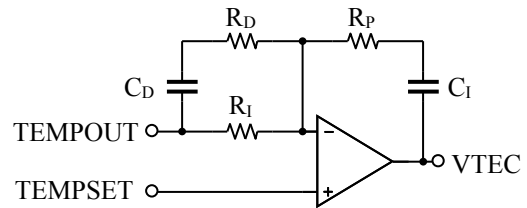
Figure 10. Compensation network
