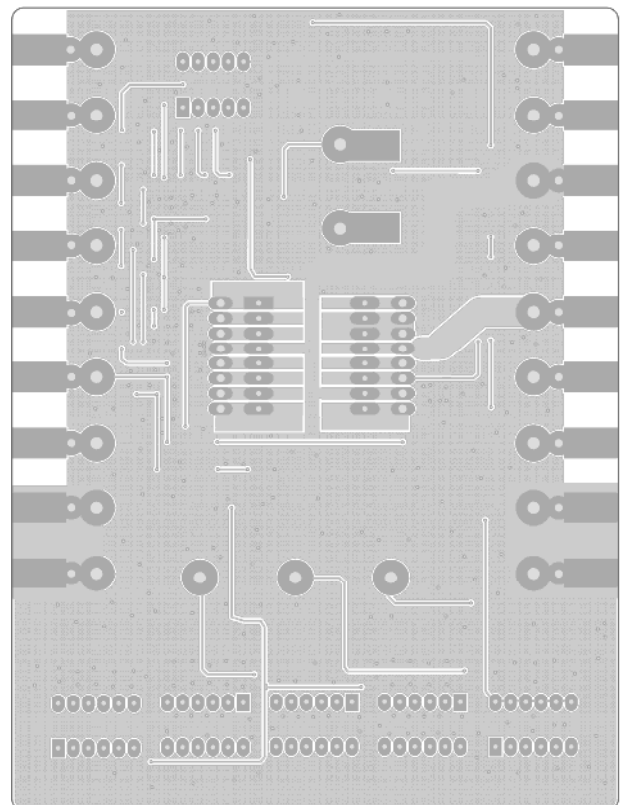
Figure 5. Bottom Layers
