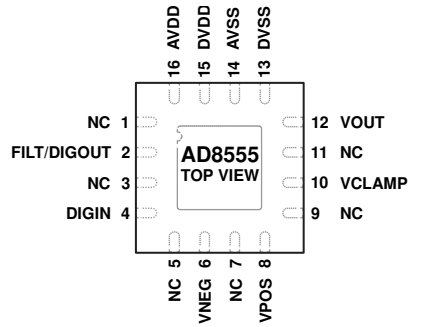
Figure 3. 16-Lead LFCSP (Not Drawn to Scale)
