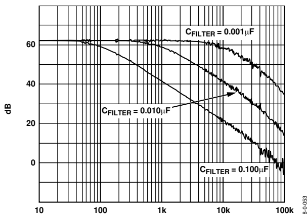
Figure 55. Typical Response of the AD8555 at FILT/DIGOUT Pin (Gain = 1280)
