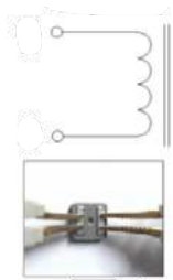
Figure 1. DCR test
