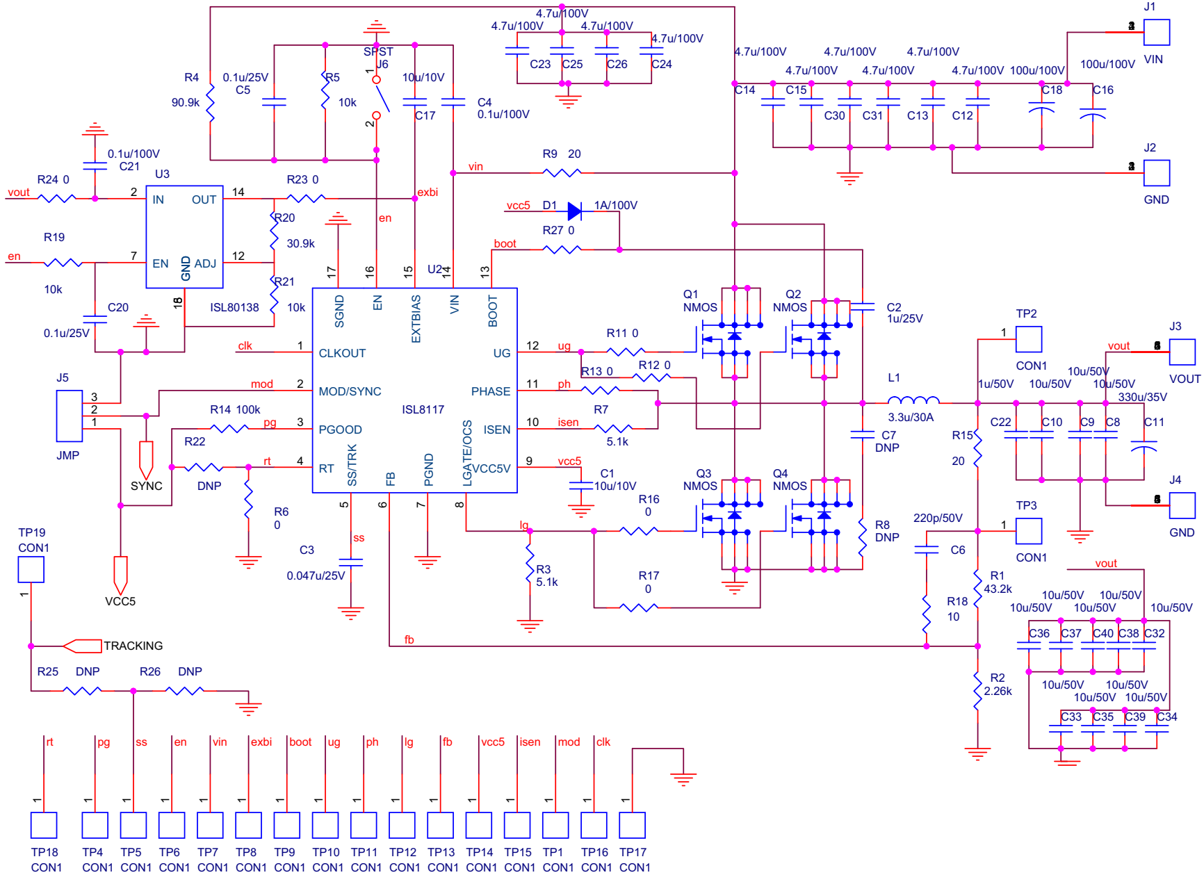
FIGURE 20. ISL8117EVAL2Z SCHEMATIC
