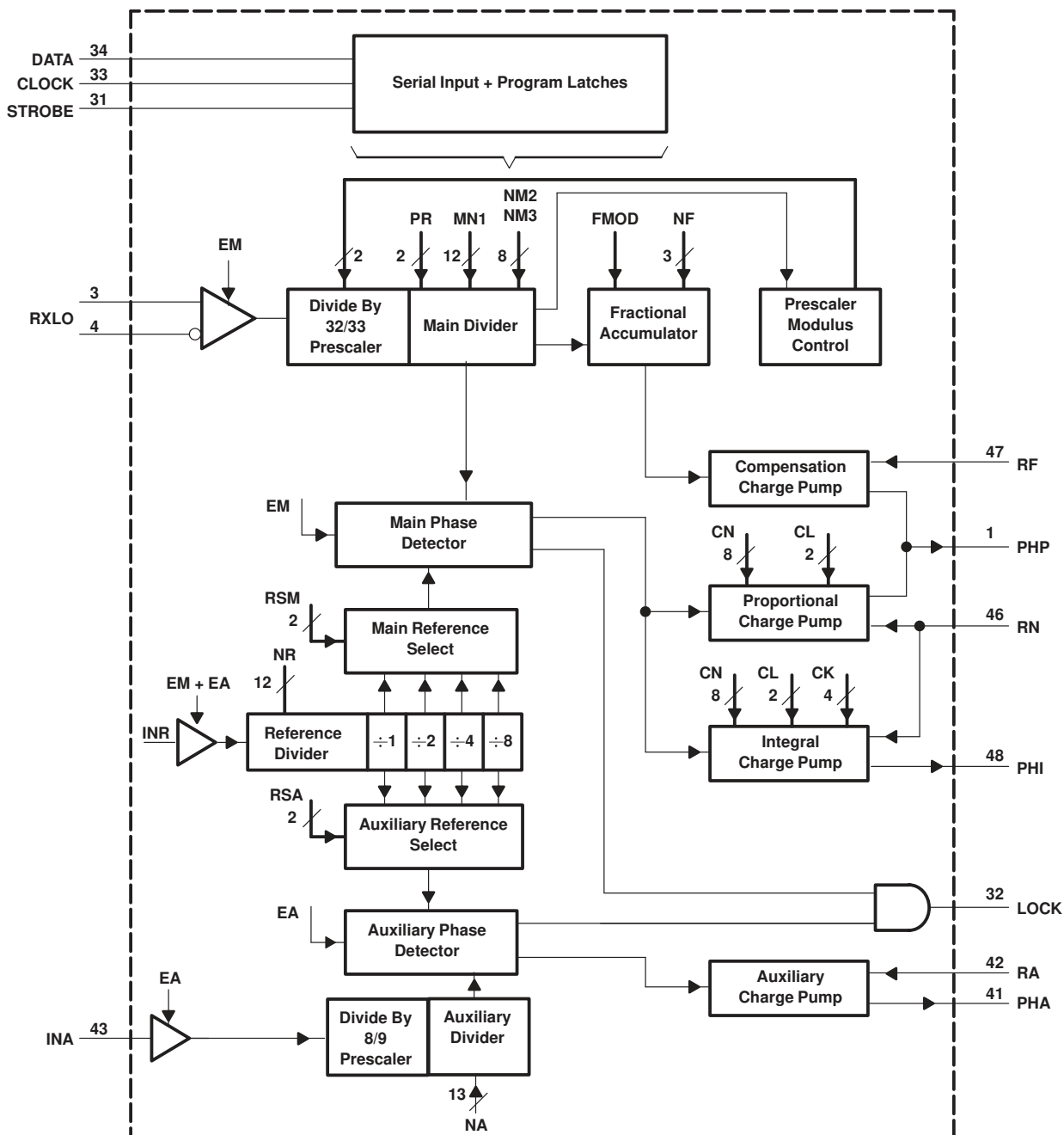
Figure 3. Frequency Synthesizer Functional Block Diagram
