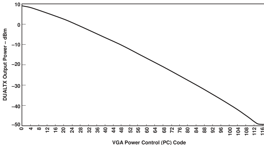
Figure 16. Power Control
