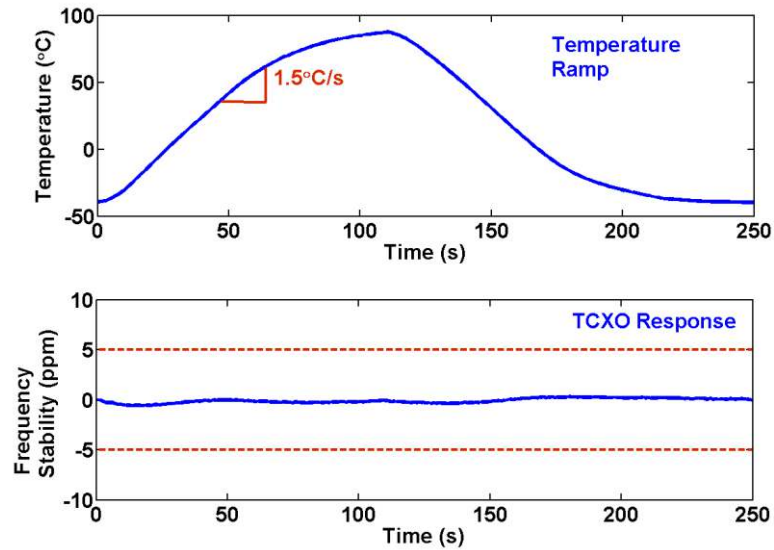
Figure 12. Temperature Ramp Response
