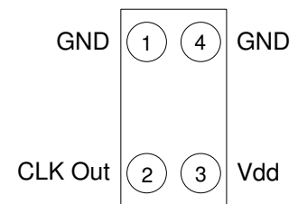
Figure 1. Pin Assignments
