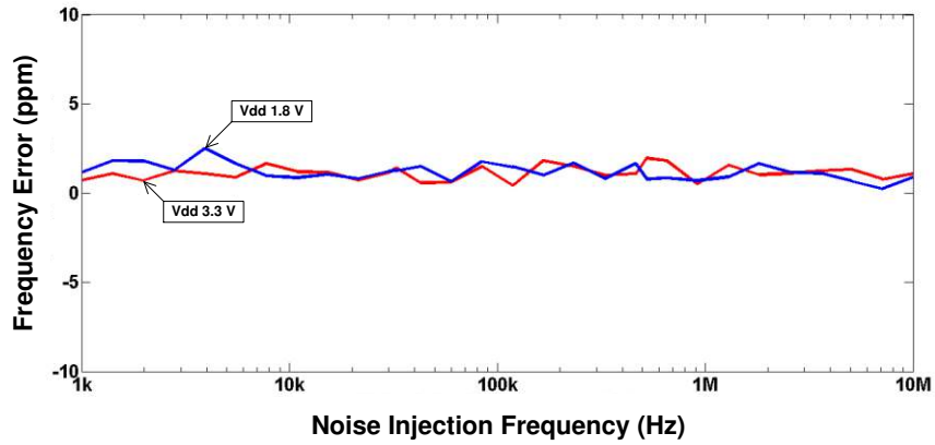
Figure 11. Power Supply Noise Rejection ( \pm 150 mV Noise)
