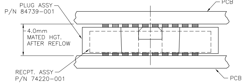
END VIEW - MATED CONNECTORS SCALE NONE
