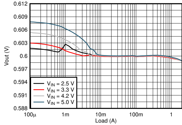
Figure 9-66. Load Regulation
