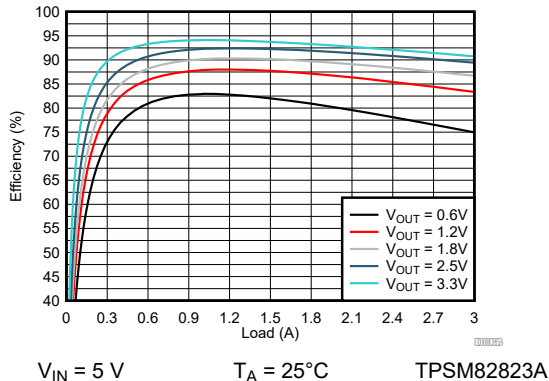
Figure 9-137. Efficiency
