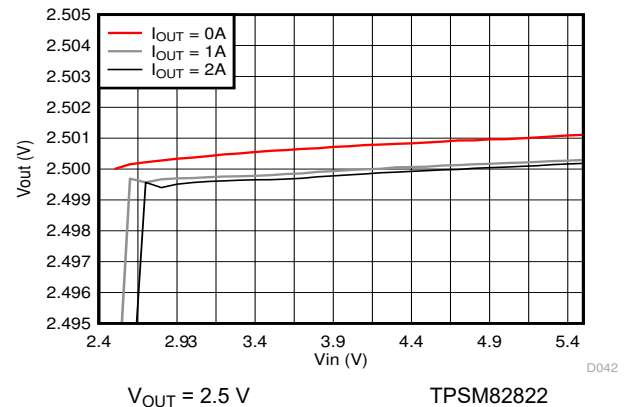
Figure 9-74. Line Regulation
