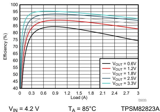
Figure 9-140. Efficiency
