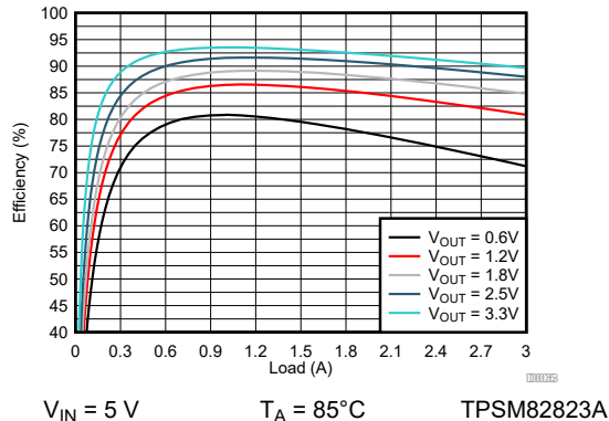
Figure 9-138. Efficiency
